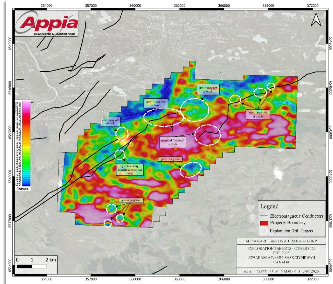
2025 exploration targets using results from the FALCON Airborne Gravity Gradiometer (AGG) & Magnetic Survey flown by Xcalibur Smart Mapping.
